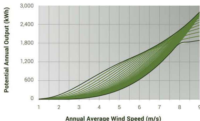
VisionAIR 3 Annual Power Output
