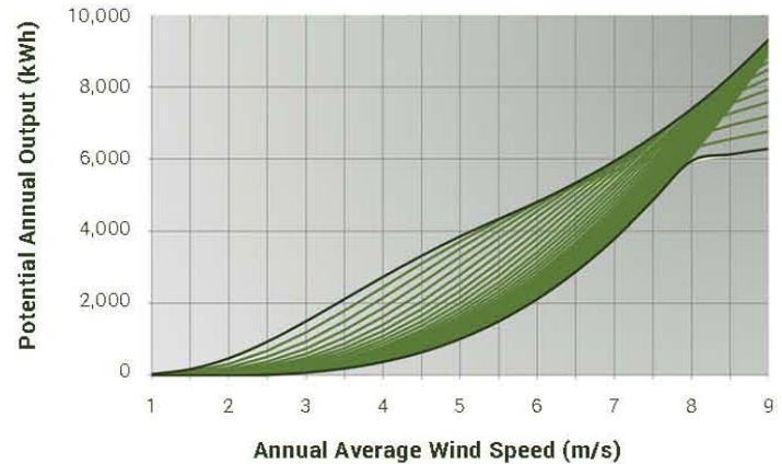
VisionAIR 5 Annual Power Output
